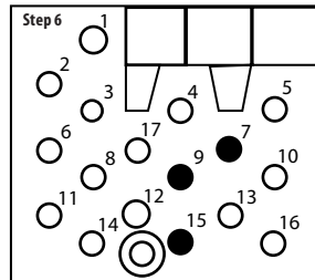
Main Connector Looking at Rear of Radio
